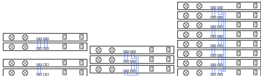
Figure 6: Illustration of the cabling of a stack of two (two or four connections), three, and eight with the XS-6128QF
