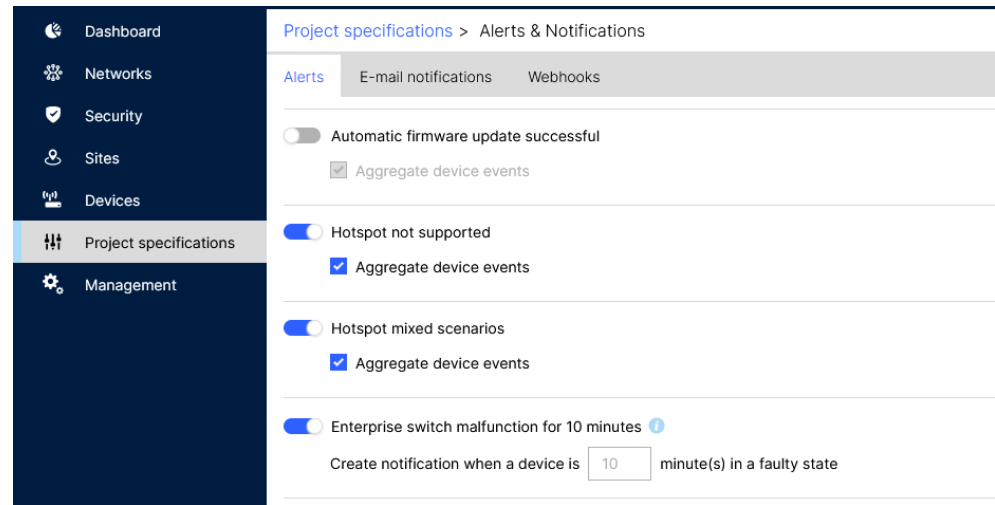
Figure 15: LMC – Configuration of warnings in the project specifications
