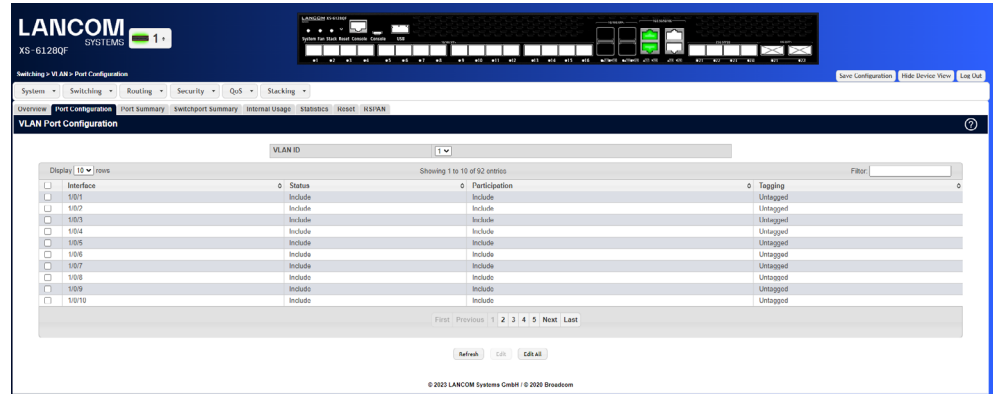
Figure 12: Port Configuration tab
