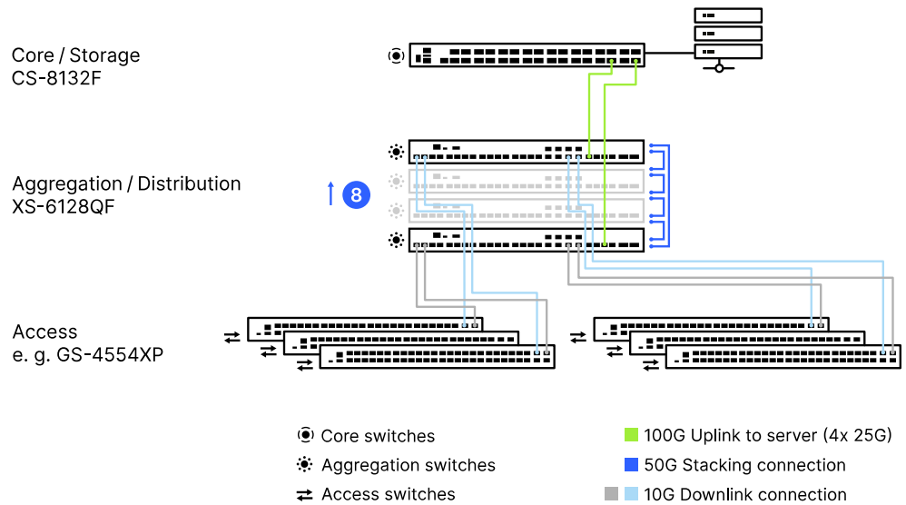
Figure 8: Network scenario with up to eight LANCOM XS-6128QF in the stack with an upper-layer core switch
