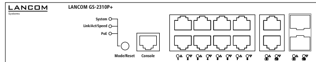
LANCOM GS-2310P+
